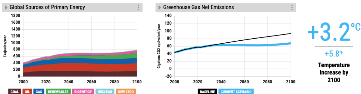
Figure 9: Default Graphs
