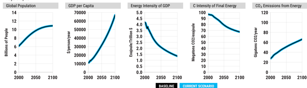
Figure 5: Kaya graphs
